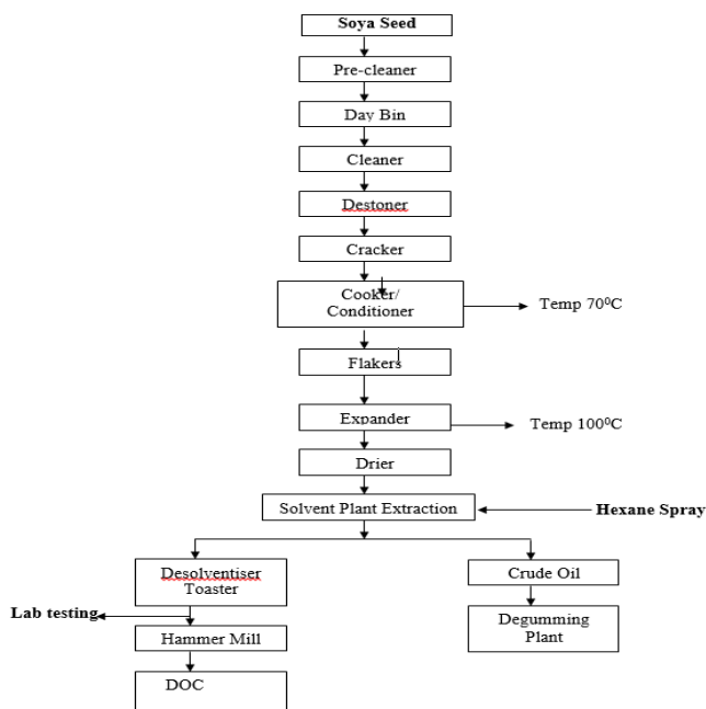
FLOW CHART FOR SOYA DOC(DEF-OILED CAKE)
